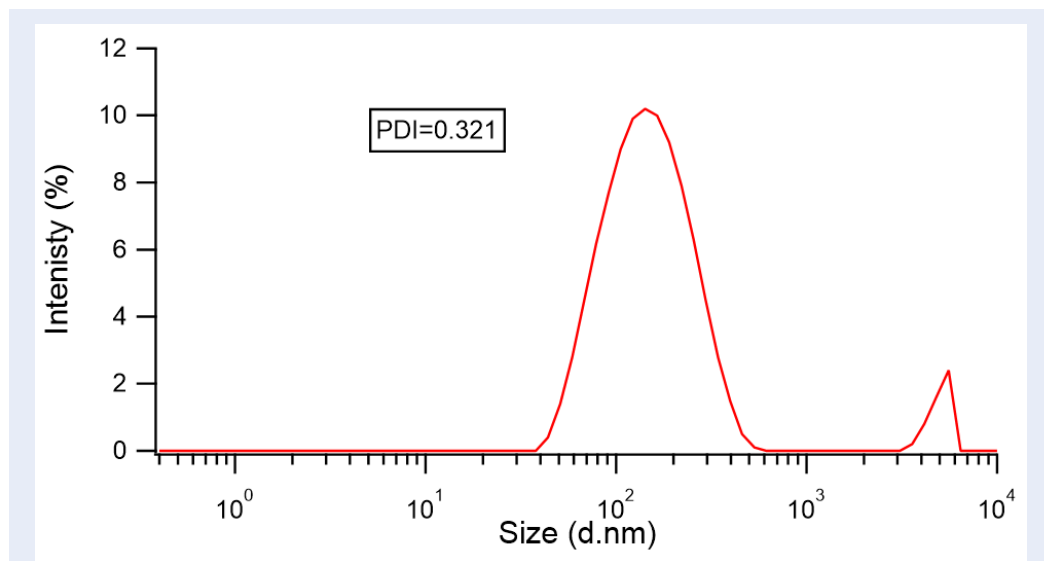
Figure S1: Particle size distribution of ZnO NPs synthesized by Fenugreek seeds aqueous extract.
